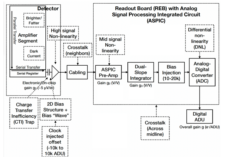
Figure 2. Schematic of the instrument model for detector effects in LSST cameras which isrTaskLSST is based on at the time of publication. Diagram made by Eli Rykoff, more details about the model can be found in https://sitcomtn-086.lsst.io/v/SITCOM-949/index.html .
