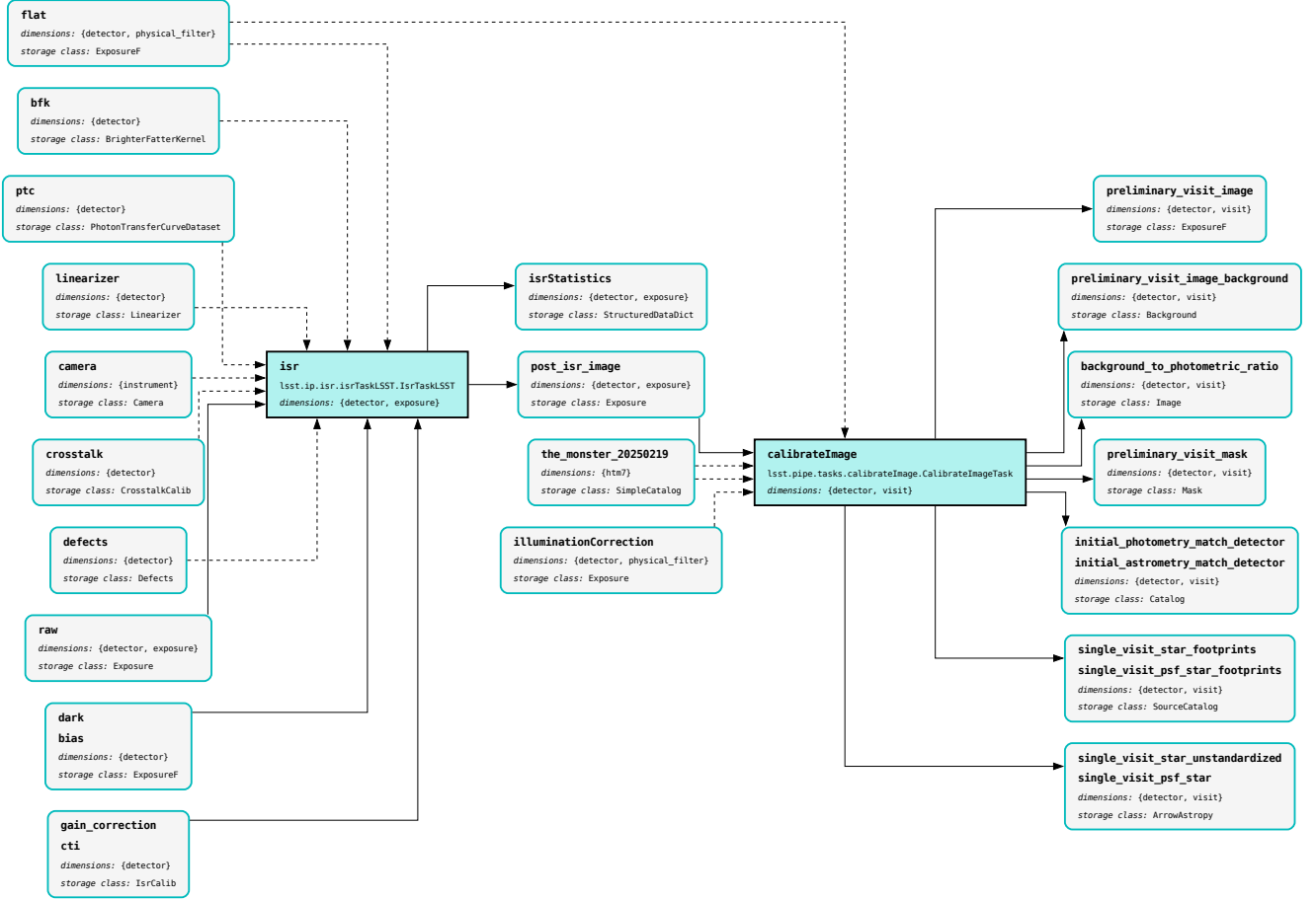
Figure 2. Example pipeline visualization of two selected tasks from the LSSTComCam/DRP-v2.yaml pipeline. The diagram illustrates the flow of datasets between tasks, with dashed lines indicating prerequisite calibration inputs. This visualization helps validate task dependencies and the expected sequence of execution.
