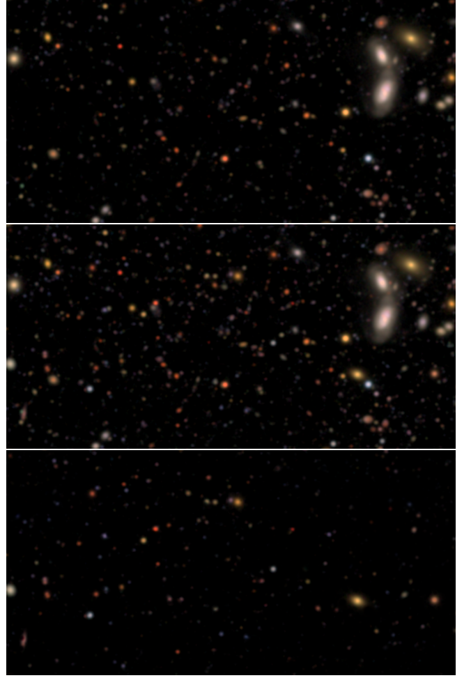
Figure 5. A LSSTComCam Data Preview 1 cutout from a deep coadd image (NSF-DOE Vera C. Rubin Observatory 2025b) at tract 5063 patch 34, with sources injected from the DC2 catalog (LSST Dark Energy Science Collaboration (LSST DESC) et al. 2021). The top panel is the original image and the middle panel shows the image with the injected sources. The bottom panel shows the difference between the two images.
