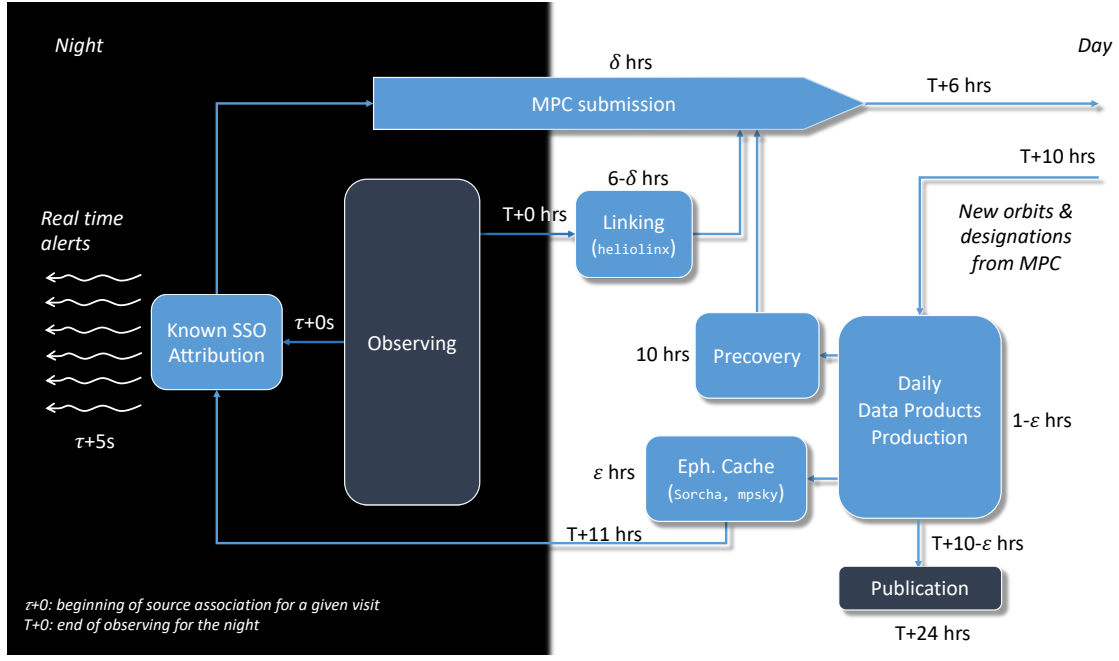
Figure 3. Detection, attribution, linking, submission and precovery of moving sources within the nightly data: The attribution is performed in real-time by the AP pipelines querying the mpsky service with resulting information attached to the alerts and queued for submission to the MPC. The linking is performed in daytime using heliolinx , with resulting links queued for submission to the MPC. Fetching of data from the MPC is performed automatically using PostgreSQL replication, with new data triggering recomputation of physical properties and precovery runs in the Daily Data Products Pipeline. Any observations discovered by the precovery procedure are queued for submission to the MPC, using the submission manager tool. The ephemeris cache is precomputed at dusk using Sorcha and mpsky , to enable fast attribution at nighttime. All timings denote design goals.
