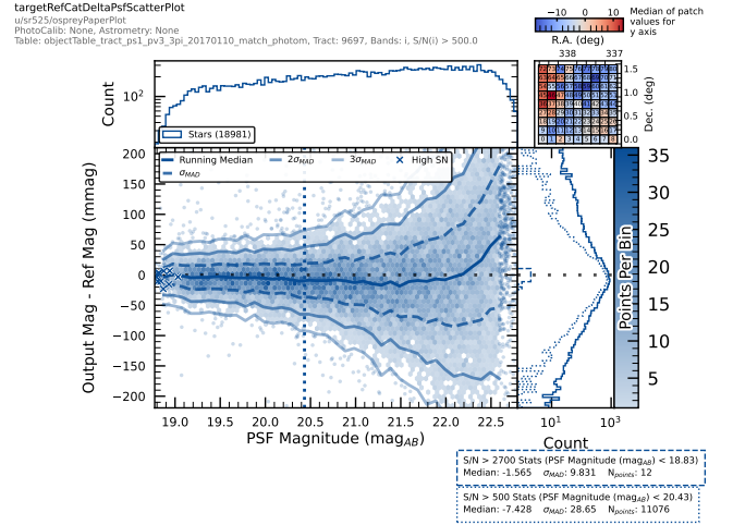
Figure 4. An example figure produced as part of the standard processing by analysis tools, the plot is information dense as it is designed for an audience familiar with the outputs but a simplified version can also be produced for talks and publications by setting a config option. The metrics shown in the bottom right of the plot are also saved separately to be displayed by various pieces of QA tooling.
