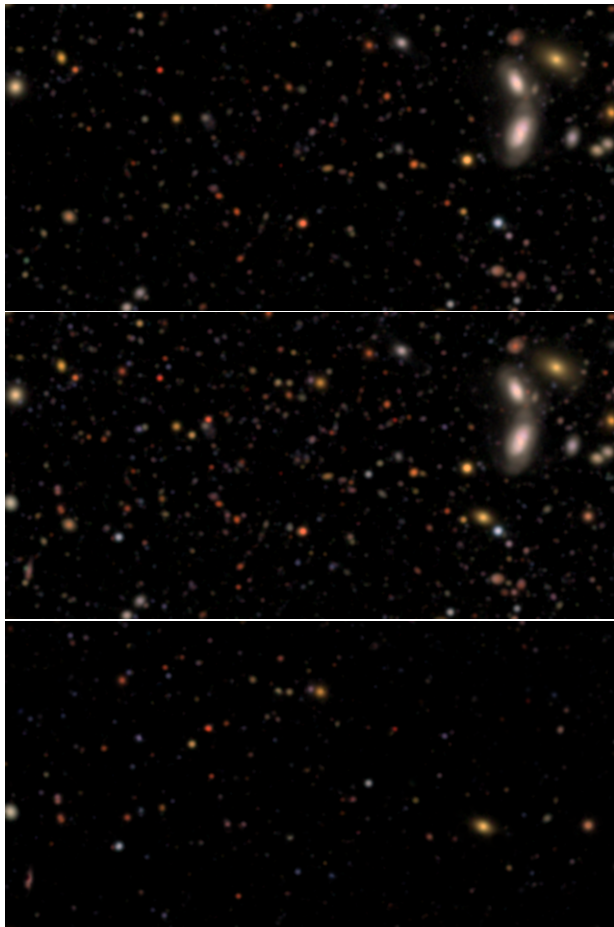
Figure 5. A LSSTComCam Data Preview 1 cutout from a deep coadd image (NSF-DOE Vera C. Rubin Observatory 2025b) at tract 5063 patch 34, with sources injected from the DC2 catalog (LSST Dark Energy Science Collaboration (LSST DESC) et al. 2021). The top panel is the original image and the middle panel shows the image with the injected sources. The bottom panel shows the difference between the two images.
