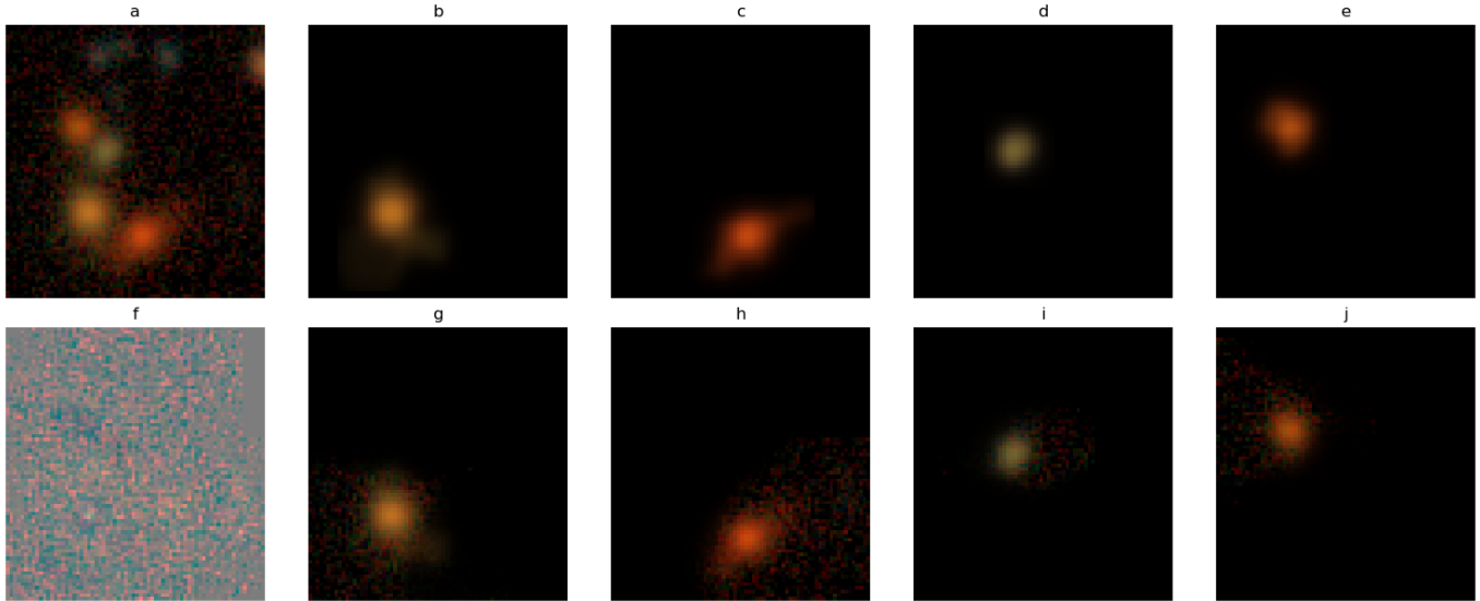
Figure 8. Example multi-object blend. The top row shows the observed multiband image (panel a) followed by the scarlet lite models of the four brightest sources (panels b through e). The bottom row shows the residual image when the scarlet lite models are subtracted from the observation (panel f) followed by the flux-conserved models (panels g through j), created by using the scarlet lite models as templates to re-distribute flux from the observation so that the total flux is conserved. The flux-conserved models, injected in a noise-replaced image, are what the science pipelines use for measurement.
