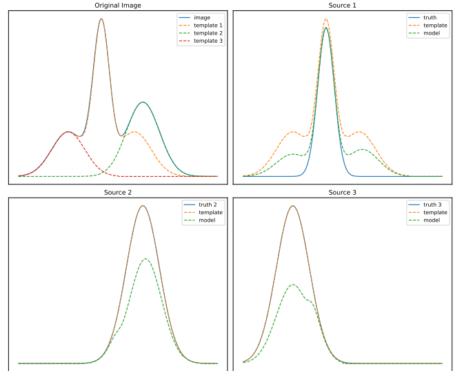
Figure 4. A 1D slice through three aligned Gaussian sources, demonstrating a failure case of relying on symmetry for generating deblender templates. Notice that for sources 2 and 3 the templates are reasonable but due to the inability of source 1 to use symmetry to constrain flux in the blended region, the resulting models for all three sources are poor. This catastrophic "three in a row" problem was part of the motivation for creating scarlet to incorporate spectral information and a more rigorous iterative deblending algorithm.
