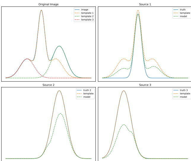
Figure 4. A 1D slice through three aligned Gaussian sources, demonstrating a failure case of relying on symmetry for generating deblender templates. Notice that for sources 2 and 3 the templates are reasonable but due to the inability of source 1 to use symmetry to constrain flux in the blended region, the resulting models for all three sources are poor. This catastrophic “three in a row” problem was part of the motivation for creating scarlet to incorporate spectral information and a more rigorous iterative deblending algorithm.
