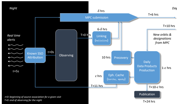
Figure 5. Detection, attribution, linking, submission and precovery of moving sources within the nightly data: The attribution is performed in real-time by the AP pipelines querying the mpsky service with resulting information attached to the alerts and queued for submission to the MPC. The linking is performed in daytime using heliolinx , with resulting links queued for submission to the MPC. Fetching of data from the MPC is performed automatically using PostgreSQL replication, with new data triggering recomputation of physical properties and precovery runs in the Daily Data Products Pipeline. Any observations discovered by the precovery procedure are queued for submission to the MPC, using the submission manager tool. The ephemeris cache is precomputed at dusk using Sorcha and mpsky , to enable fast attribution at nighttime. All timings denote design goals.
