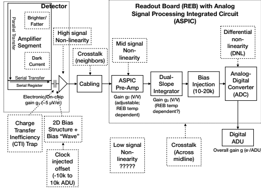
Figure 3. Schematic of the instrument model for detector effects in LSST cameras which isrTaskLSST is based on at the time of publication. More details about the model can be found in P. Fagrellius & E. Rykoff (2025) and A. A. Plazas Malagón et al. (2024).
