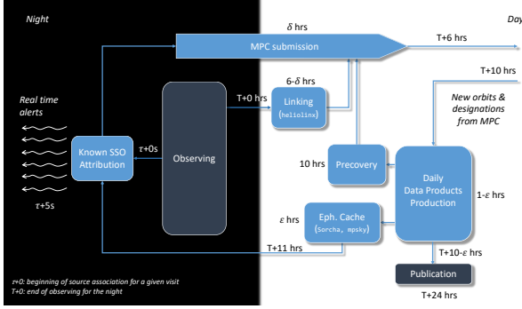
Figure 5. Detection, attribution, linking, submission and precovery of moving sources within the nightly data: The attribution is performed in real-time by the AP pipelines querying the mpsky service with resulting information attached to the alerts and queued for submission to the MPC. The linking is performed in daytime using heliolinx , with resulting links queued for submission to the MPC. Fetching of data from the MPC is performed automatically using PostgreSQL replication, with new data triggering recomputation of physical properties and precovery runs in the Daily Data Products Pipeline. Any observations discovered by the precovery procedure are queued for submission to the MPC, using the submission manager tool. The ephemeris cache is precomputed at dusk using Sorcha and mpsky , to enable fast attribution at nighttime. All timings denote design goals.
