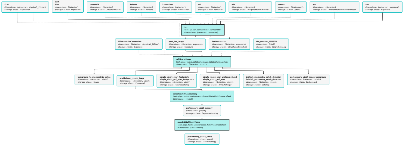
Figure 2. Example pipeline visualization of four selected tasks from the LSSTComCam/DRP-v2.yaml pipeline in the Mermaid format. The diagram illustrates the flow of datasets between tasks, with dashed lines indicating prerequisite inputs. This visualization helps validate task dependencies and the expected sequence of execution.
